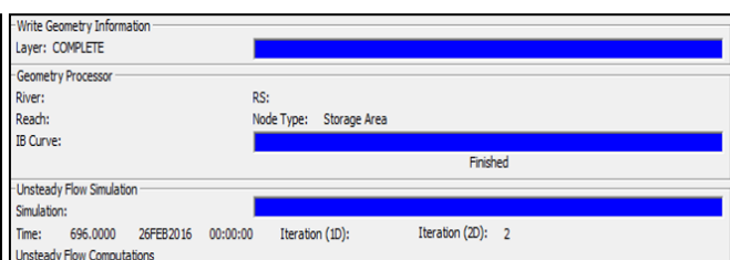
Figure 3.7: HEC-RAS computation.
