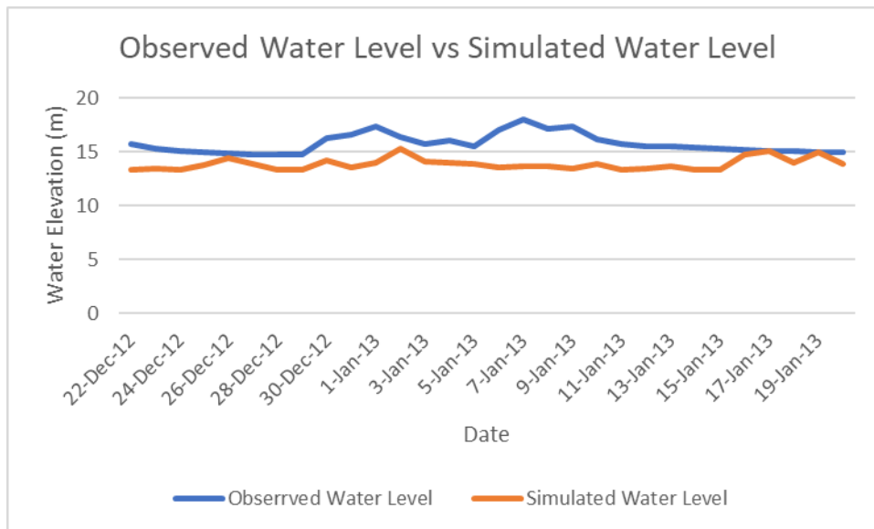
Figure 4.2: Observed Water Level vs Simulated Water Level for 2nd Calibration.
