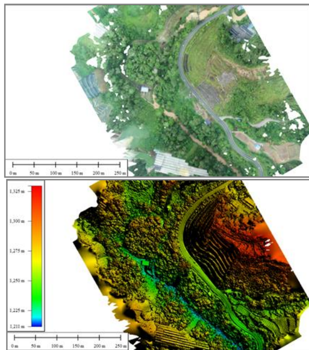
Figure 5. Orthoimage (left) and Digital Surface Model, DSM (right) based on Drone Mapping
