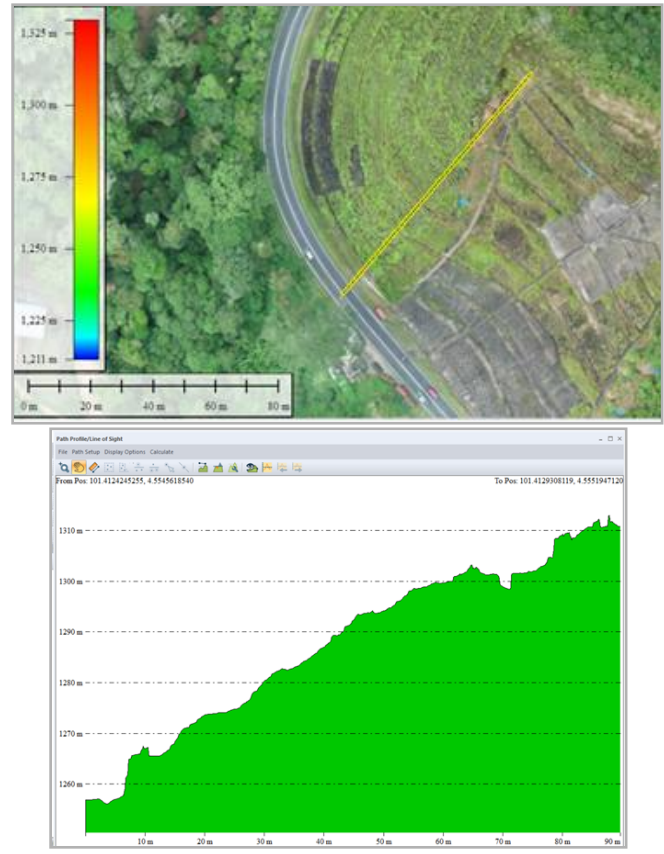
Figure 6. Cross-Section of Terrain Slope
