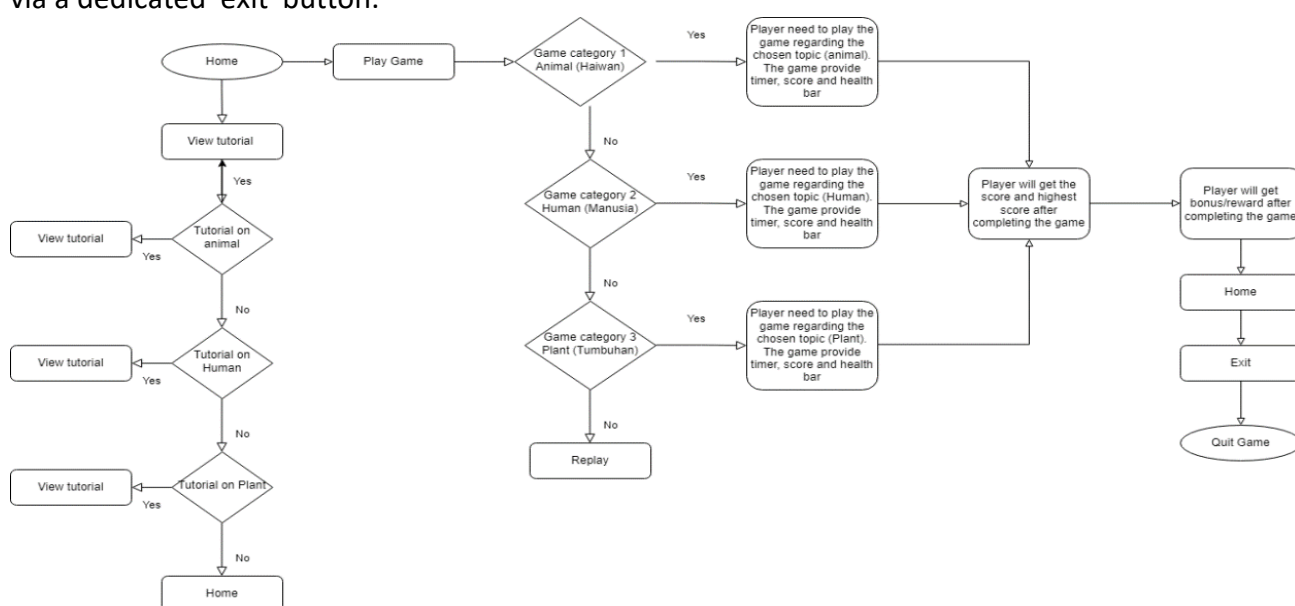
Fig. 2 Application flowchart
