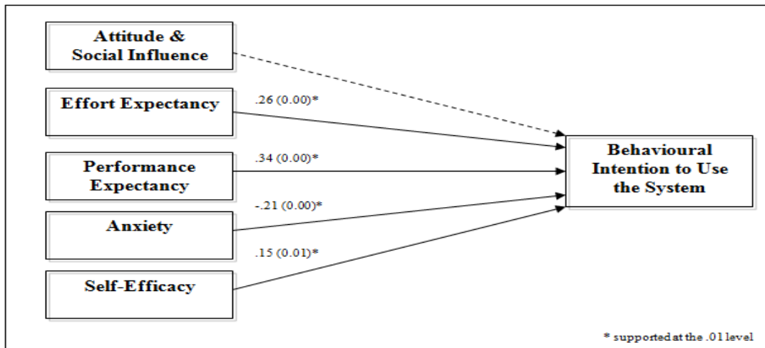
Figure 1: Research Model
