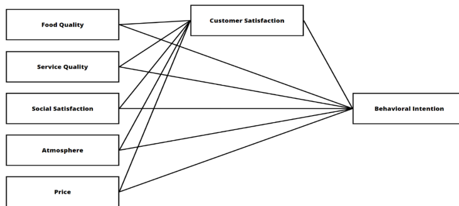
Figure 2. Conceptual Framework
