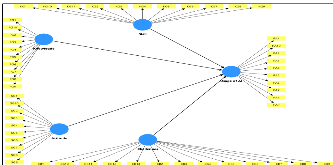
Figure 1. Preliminary SmartPLS 4 Model Showing Relationships Among Knowledge, Skills, Attitude, Challenges, and (AI) Usage Level.
