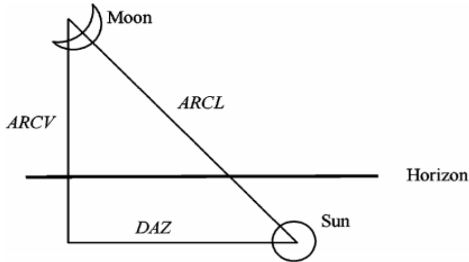
Figure 1: Important variables for crescent visibility during observation (Odeh, 2004)
