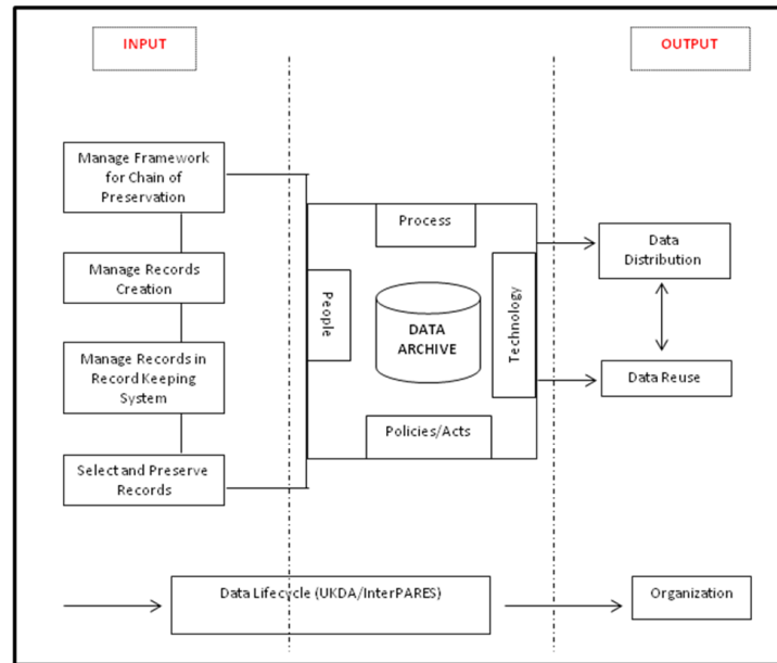
Fig. 4. Second Level of Primary Research Data Preservation Framework.
