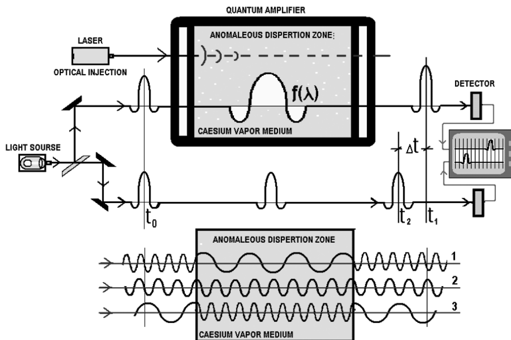
Figure 5. Experiments of L.Wang - superluminal light propagation.
