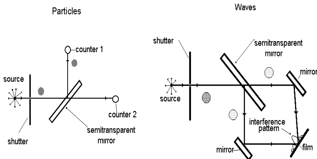
Figure 1. Experiments with individual photons on semitransparent mirror.
