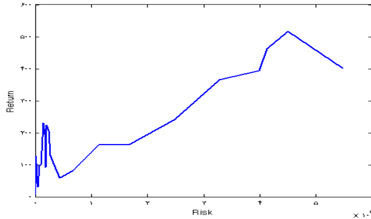
Figure 4. The relationship between risk and return in the implementation of the algorithm by table 4 parameters
