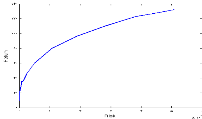
Figure 3. The relationship between risk and returns in the implementation of the algorithm by table 3 parameters
