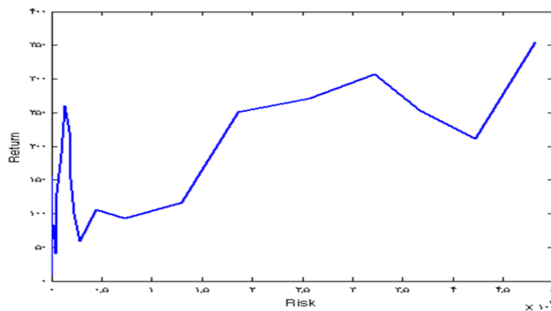
Figure 5. The relationship between risk and return in the implementation of the algorithm by table 5 parameters
