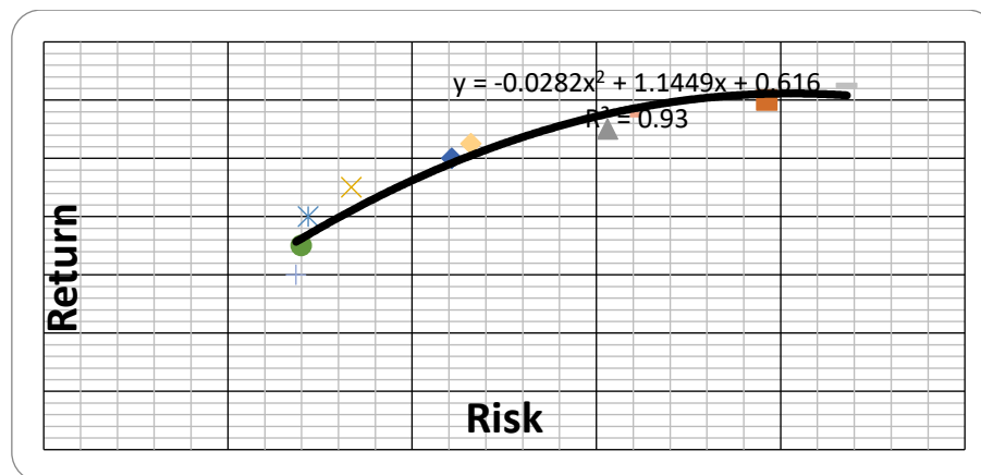
Figure 8. Obtained efficient set in mean – variance method of the implementation Birds Flight algorithm
