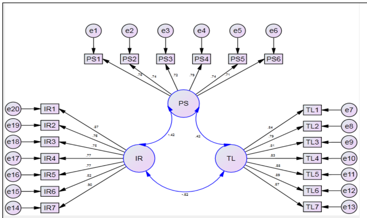
Figure 2: Analytical model Goodness of Fit Indices of Measurement Model
